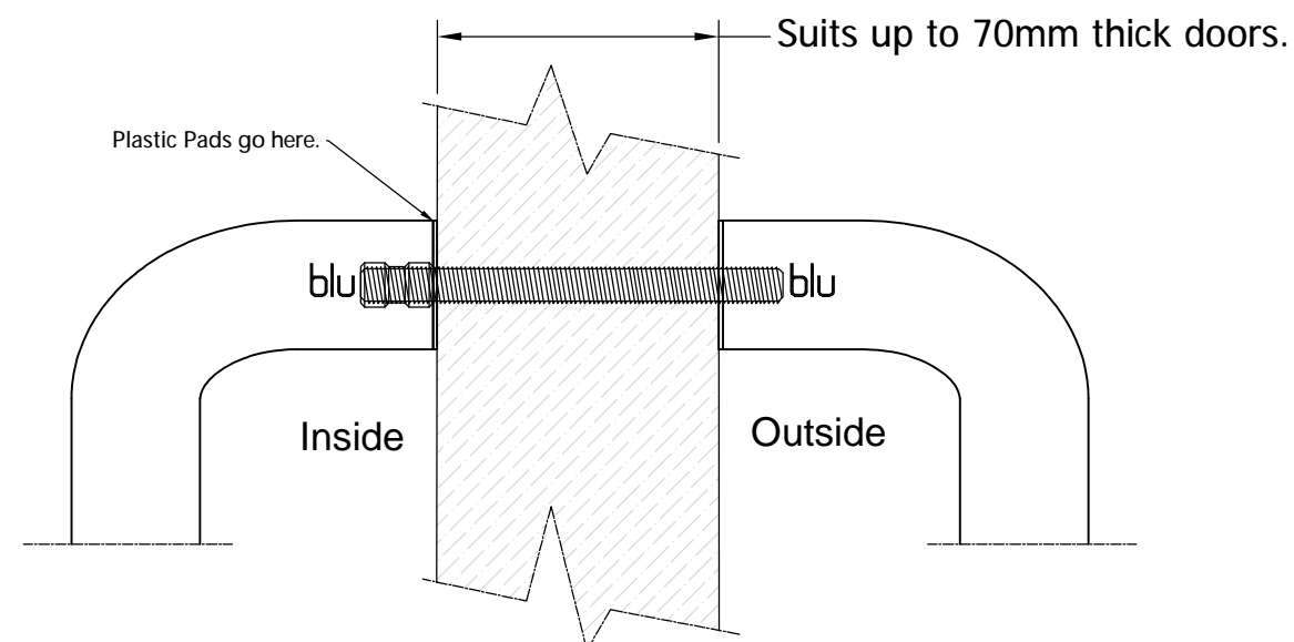
Assembled View (Back to Back Fix)
