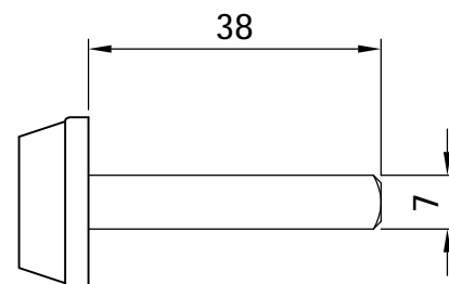
SPINDLE DIMENSIONS
