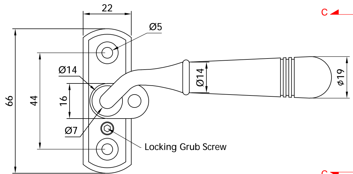
Section B-B FRONT VIEW - OPEN POSITION
