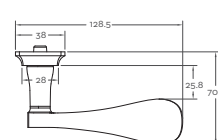
Top Profile
