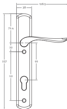
Front Profile
