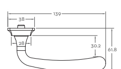
Top Profile
