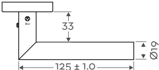
Top Profile
