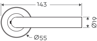
Front Profile
