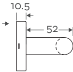
Side Profile
