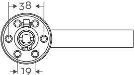
Rear Profile
