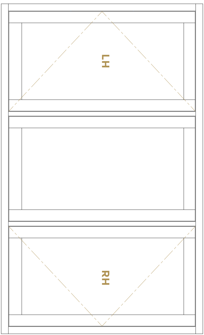
FH Tritus Lift-Off Butt Hinge, viewed from the outside.
