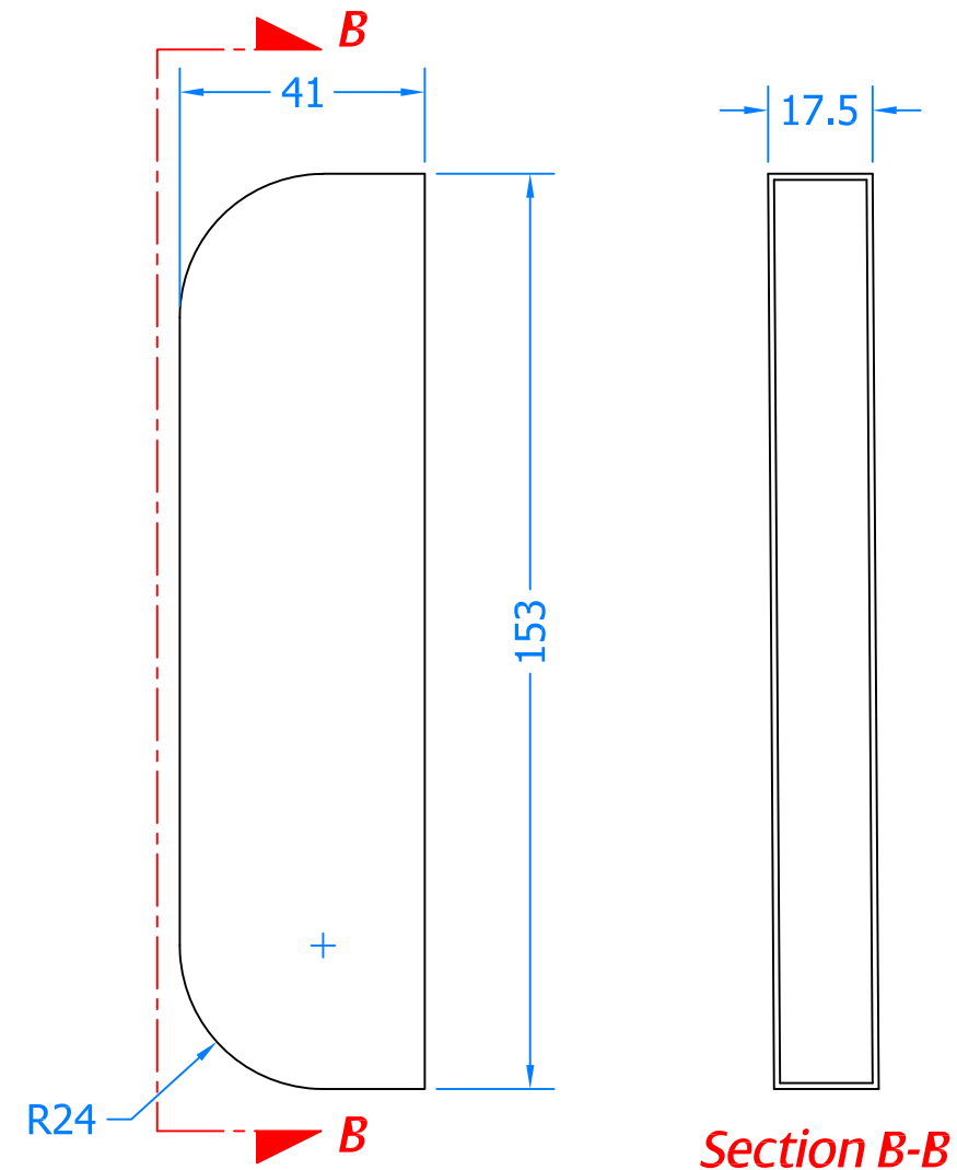
Top/Bottom Gearbox Cover
