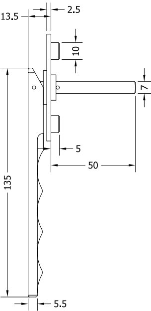
Side Profile
