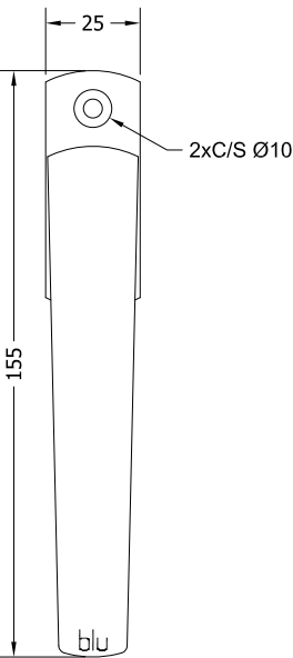
Front Profile
