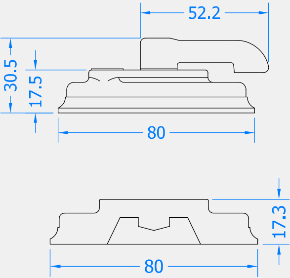
Front Profile
