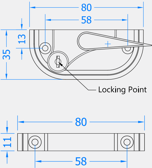
Top Profile
