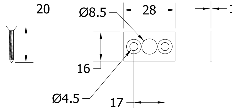
Flat Plate Keep
