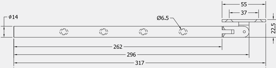
Front Profile SST91
