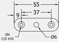
Top Profile Pin
