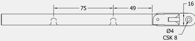
Top Profile SST93
