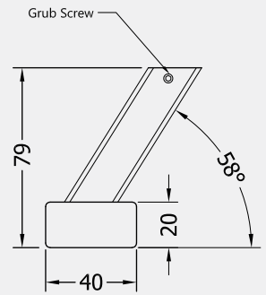
Top Profile
