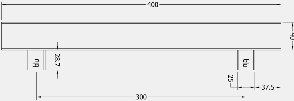
Side Profile
