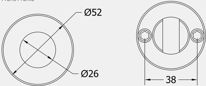
Front Profile
