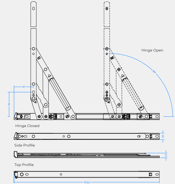
Hinge Project Out Dimension
