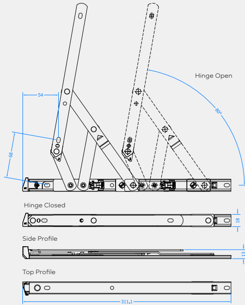
Hinge Project Out Dimension
