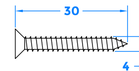
6 x 4x30 Woodcrews
