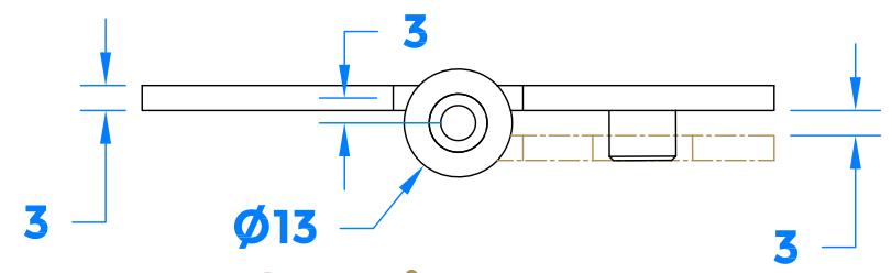
Section A-A Top View
