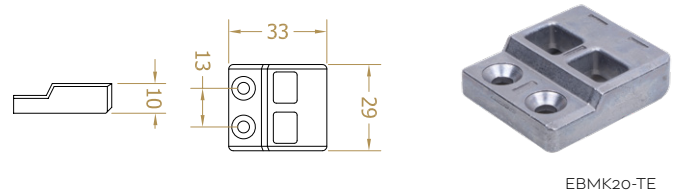
EBMK20-TE
