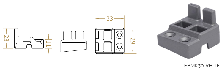
EBMK30-RH-TE
