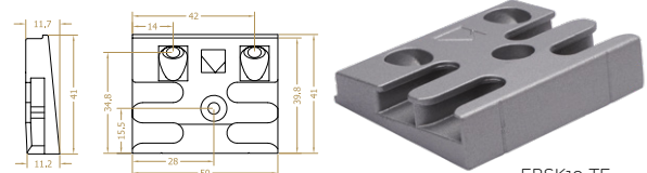
EBSK10-TE
