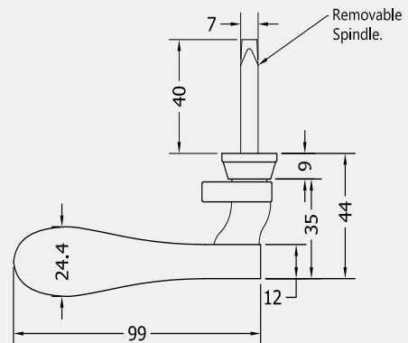
Top Profile
