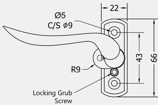
Front Profile
